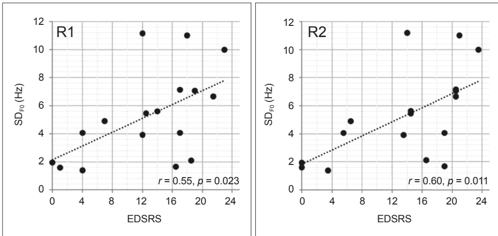
Supplementary Figure 3. Scatter plots of correlation analyses performed for assessment of convergent validity between average ratings of reviewers 1 and 2 (R1, R2) and the F0 variability (SD F0 ). Significance level for the Pearson correlation analyses was set at p < 0.025 (0.05/2, Bonferroni-corrected). EDSRS, Embouchure Dystonia Severity Rating Scale.
